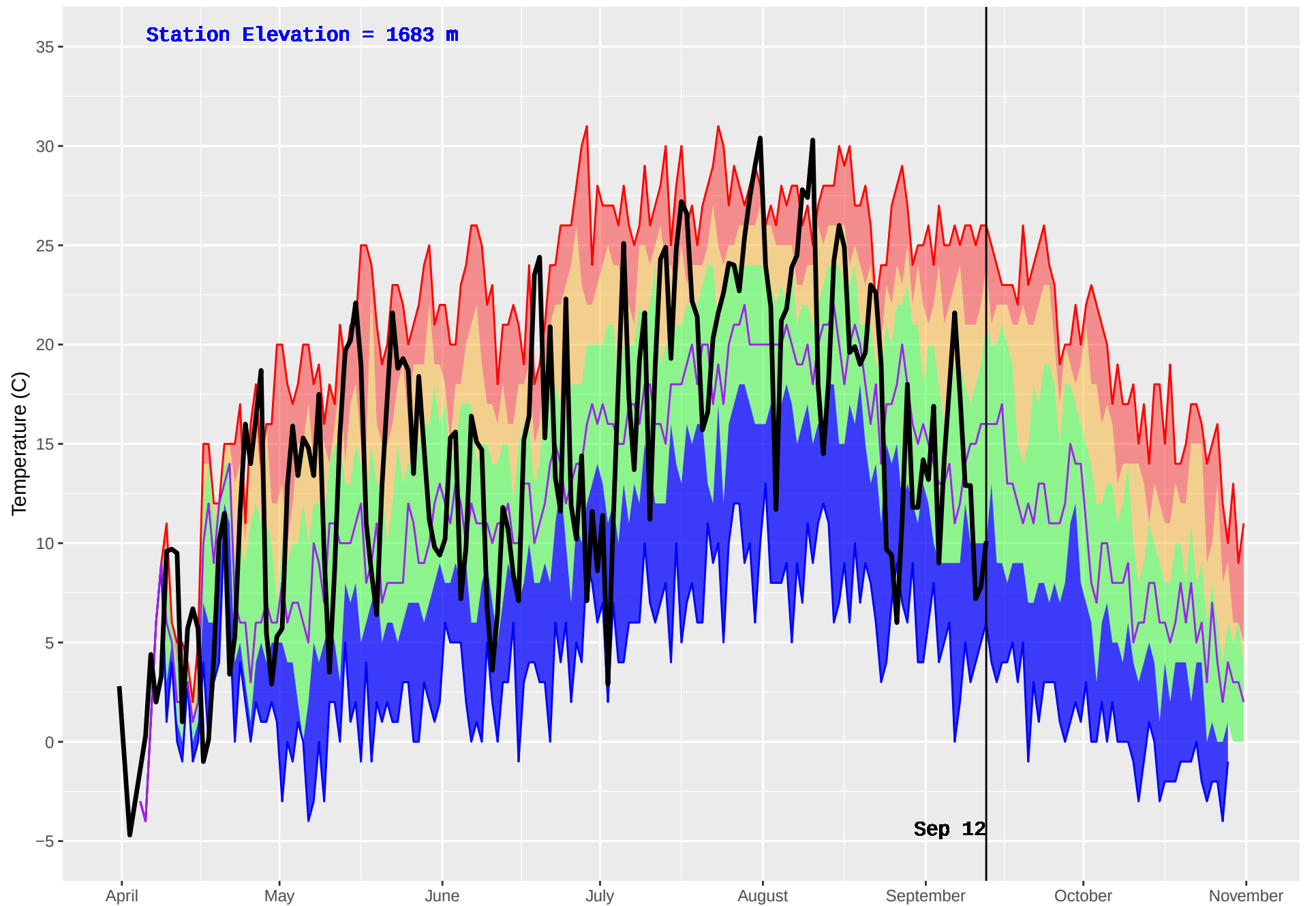
ASHNOLA (331) : Historical (1992–2016) and Current (2018) Daily Temperature
